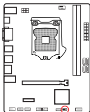
2-1 Clear CMOS Jumper CLR-CMOS
