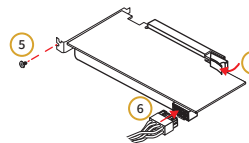
2-9 Graphics Card Installation
