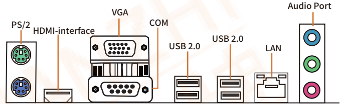
1-2 Overall Rear I/O Panel Display
